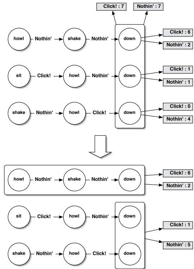
Figure 2: OFESI action splitting method for synthetic characters
